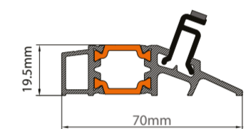
EAVES BEAM ASSEMBLY
