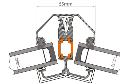
GEORGIAN HIP RAFTER ASSEMBLY
