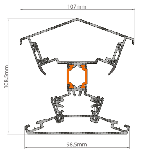
RIDGE ASSEMBLY
