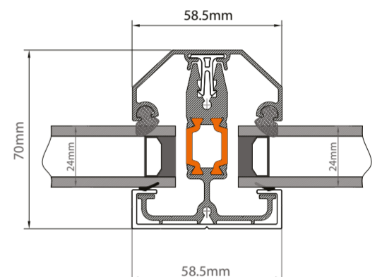
RAFTER ASSEMBLY
